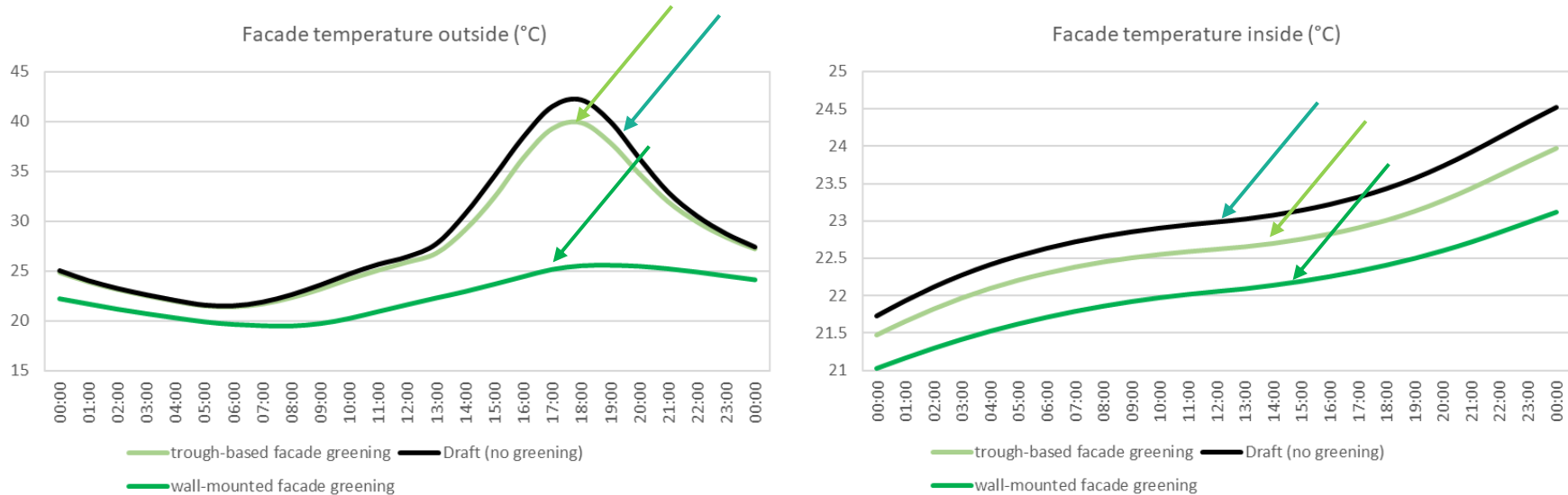
Comparison of façade temperature outside (a) and inside (b) with/without façade greening within one day
