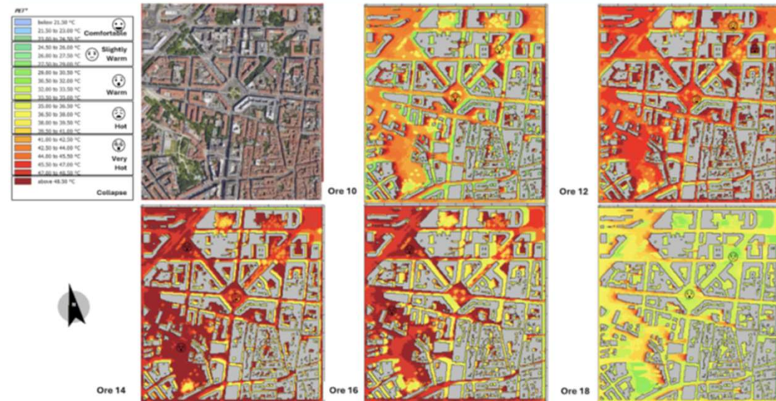
Results PET (°C) Physiological Equivalent Temperature
